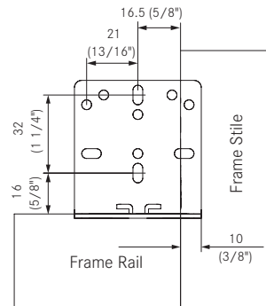
Rear Bracket for Face Frame
